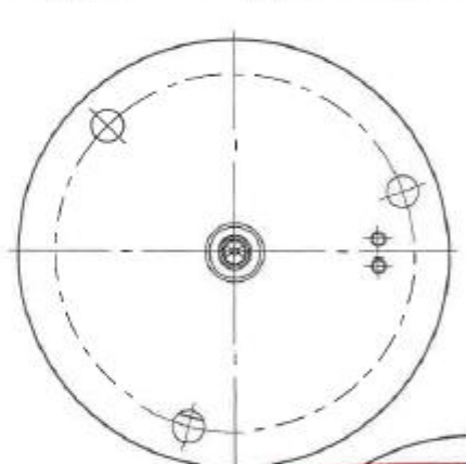
ITEM 2 CLAMP UNIT MATERIAL: ST. STEEL 316 QTY: 1 WEIGHT: 0.1 kg SCALE: 1:1
