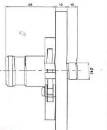
ITEM 1 BRUSH COUPLING MATERIAL: ST. STEEL 316 QTY: 1 WEIGHT: 1.3 kg SCALE: 1:1
